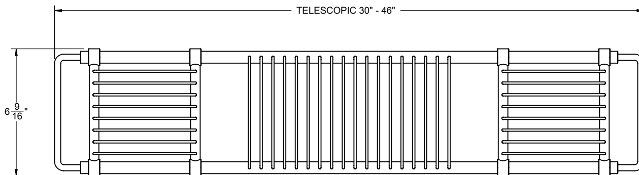
TOP VIEW
